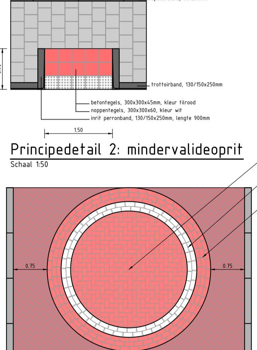
Principedetail 2: mindervalideoprit Schaal 1:50
