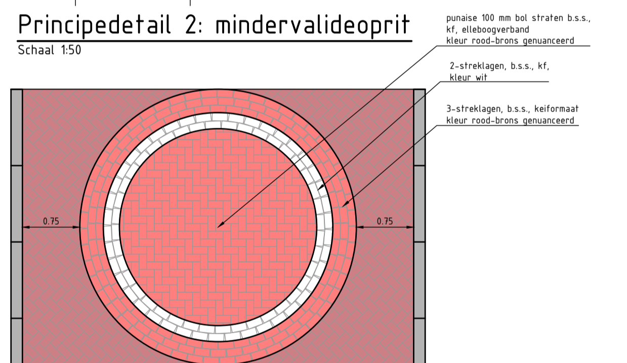
Principedetail 2: mindervalideoprit Schaal 1:50
